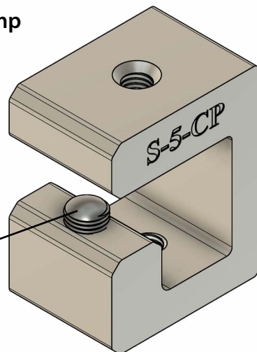
Setscrew
