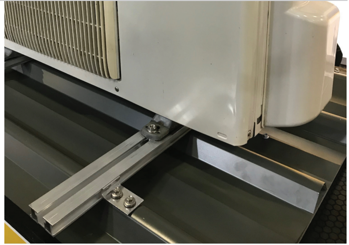
Use this detail with profiles such as TRIMDEK ®
